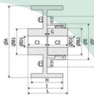
BRAKE DRUM WITH GEAR COUPLING
