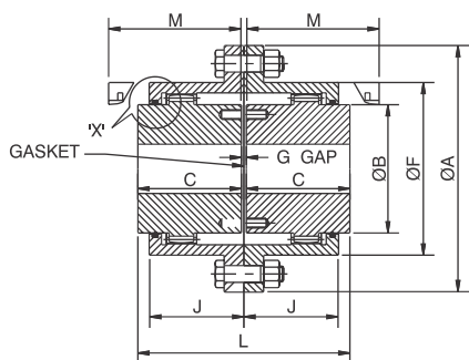
FULL GEAR COUPLE
