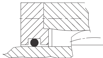
DETAIL 'X' THIS COVER PLATE CONSTRUCTION FOR SIZES FG - 111 ONWARDS
